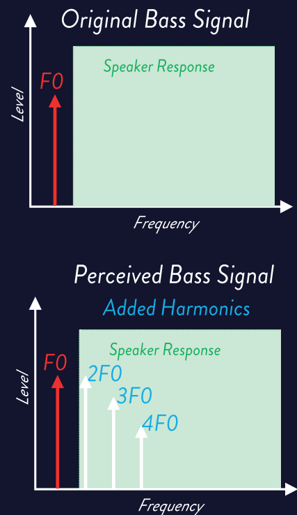
Virtual Bass
