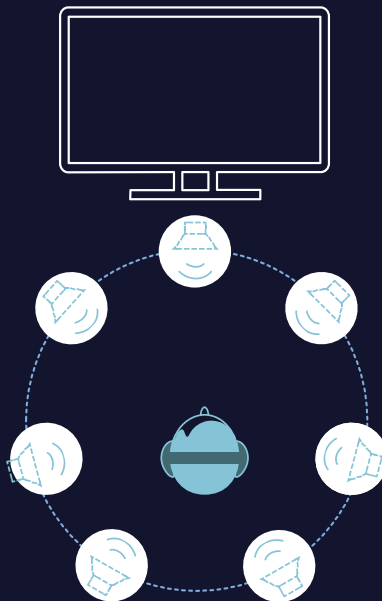
Headphone Virtualizer
